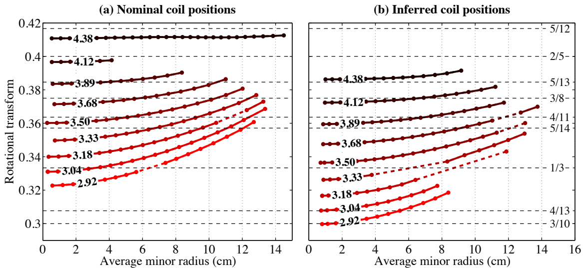
Figure 14. Comparison of t profiles calculated for selected current-ratios in the nominal and optimized coil configurations. (a) Profiles for the nominal IL coil positions ( \mathbf{p}_0 ) and assuming no PF coil displacements, identical to what is plotted in Fig. 3. (b) Profiles computed using the optimized IL coil configuration ( \mathbf{p}_{3.68}^* ) and the measured PF coil displacements. Each dot represents a closed flux surface, so while the curves for I_{IL}/I_{PF} = 3.04 and 2.92 in plot (b) do not pass through t = 1/3 , they contain large three-island chains on their edges. Note that, in the optimized configuration (b), current-ratios I_{IL}/I_{PF} less than 3.5 contain t = 1/3 , consistent with observations.
