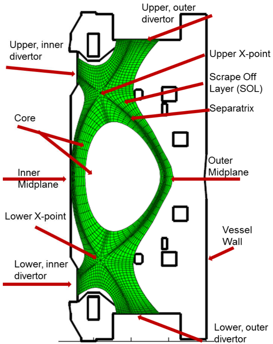
Figure 2: The mesh used for SOLPS simulations of MAST.
