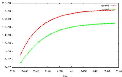
Figure 4: Density calculated using the SOLPS-Eirene package (fine solver). The parareal computation matches this solution.
