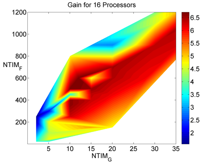
Figure 10: The parareal gain depends on the number of timesteps ( NTIM_F for fine and NTIM_G for coarse) solved per processor.
