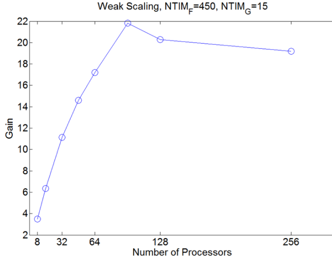
Figure 12: Weak scaling studies. Here NTIM_F = 450 and NTIM_G = 15 .
