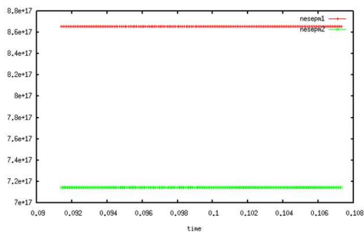
Figure 5: Density computed using the coarse solver (Eirene replaced by fluid neutral model) is different from the fine solution.
