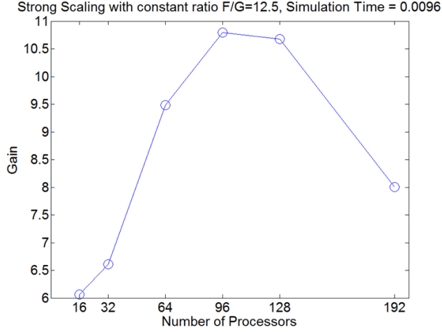
Figure 13: Strong scaling studies. The gain decreases at high processor count when the size of the time slice solved per processor is significantly reduced.
