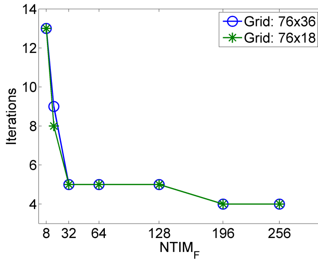
Figure 11: For the same number of timesteps solved per processor for the coarse computation, the parareal iteration k required for convergence depends on the number of timesteps used for the fine computation ( NTIM_F ).
