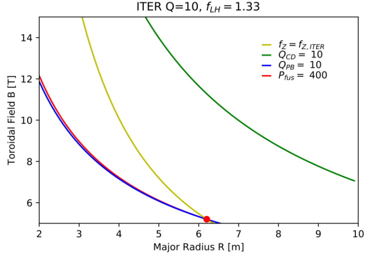
Fig. 1: Lines of constant figures of merit in R - B space for the ITER scenario ( A=3.1 , q=3.1 , H=1 , \beta_N=1.8 , f_{GW}=0.85 , f_{LH}=1.33 ). The red point shows the ITER design point.
