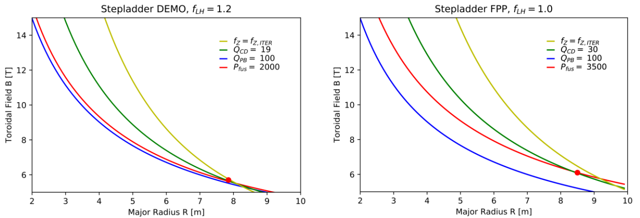
Fig. 2: Lines of constant figures of merit in R - B space for the stepladder scenario ( A=3.1 , q=4.5 , H=1.2 , \beta_N=3.5 , f_{GW}=1.2 ). The red point shows the DEMO (left diagram) and the FPP (right diagram) design points.
