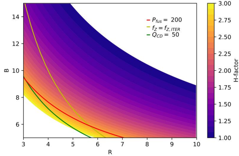
Fig. 4: Lines of constant figures of merit in R - B space for relaxed physics assumptions w.r.t. the stepladder scenario ( A=3.1 , \beta_N=3.0 , f_{GW}=1.0 ). For the operational space opening up at low R , high B , the H-factor, shown as contours, has to be quite high.
