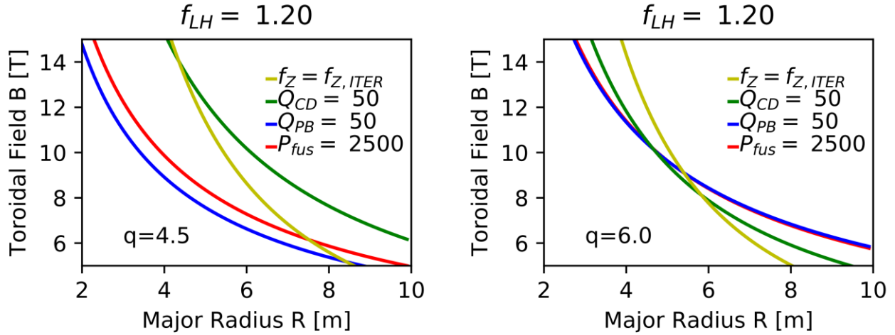
Fig. 3: Lines of constant figures of merit in R - B space for the stepladder scenario ( A=3.1 , H=1.2 , \beta_N=3.5 , f_{GW}=1.2 ). At q = 4.5 (left), it is not possible to find a solution at high Q_{CD} = 50 up to B = 15 T, but increasing q to 6 opens up a parameter space above 9.5 T for such a solution.
